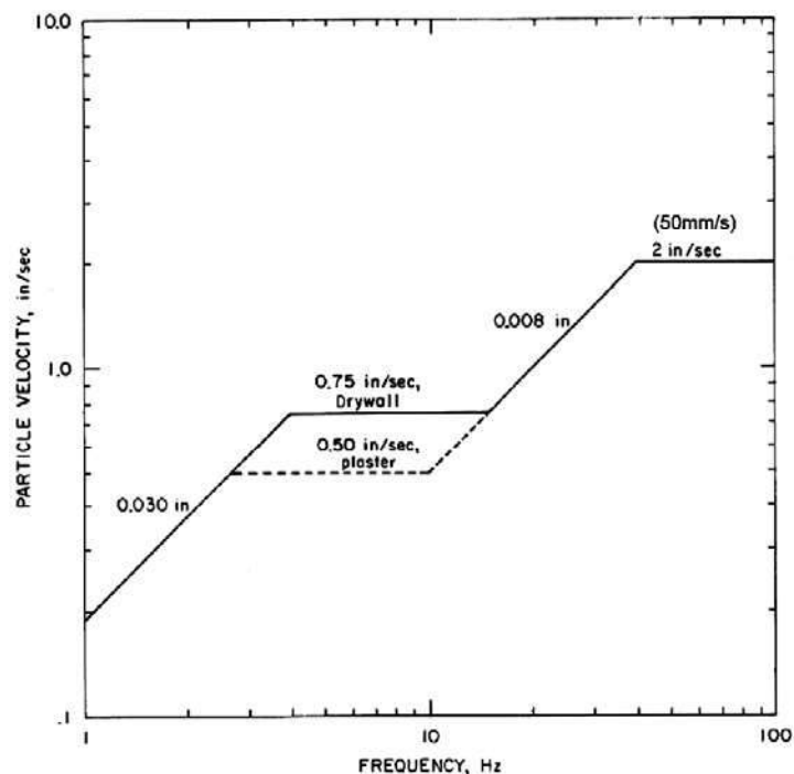
Figure 1 – USBM Z-Curve
